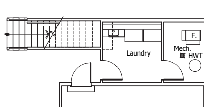
PARTIAL FIRST FLOOR PLAN W/ SLAB (W/ SECOND FLOOR)
