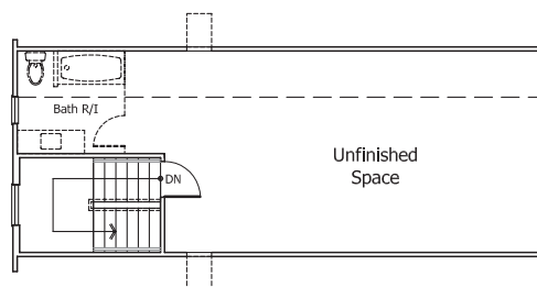
UNFINISHED SECOND FLOOR
