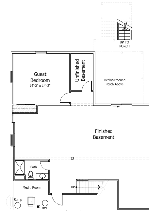
LOWER LEVEL FINISHED BASEMENT W/ WALKOUT
