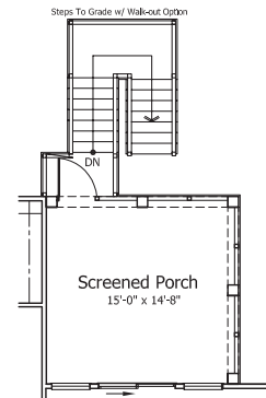
REAR SCREENED PORCH W/ WALKOUT
